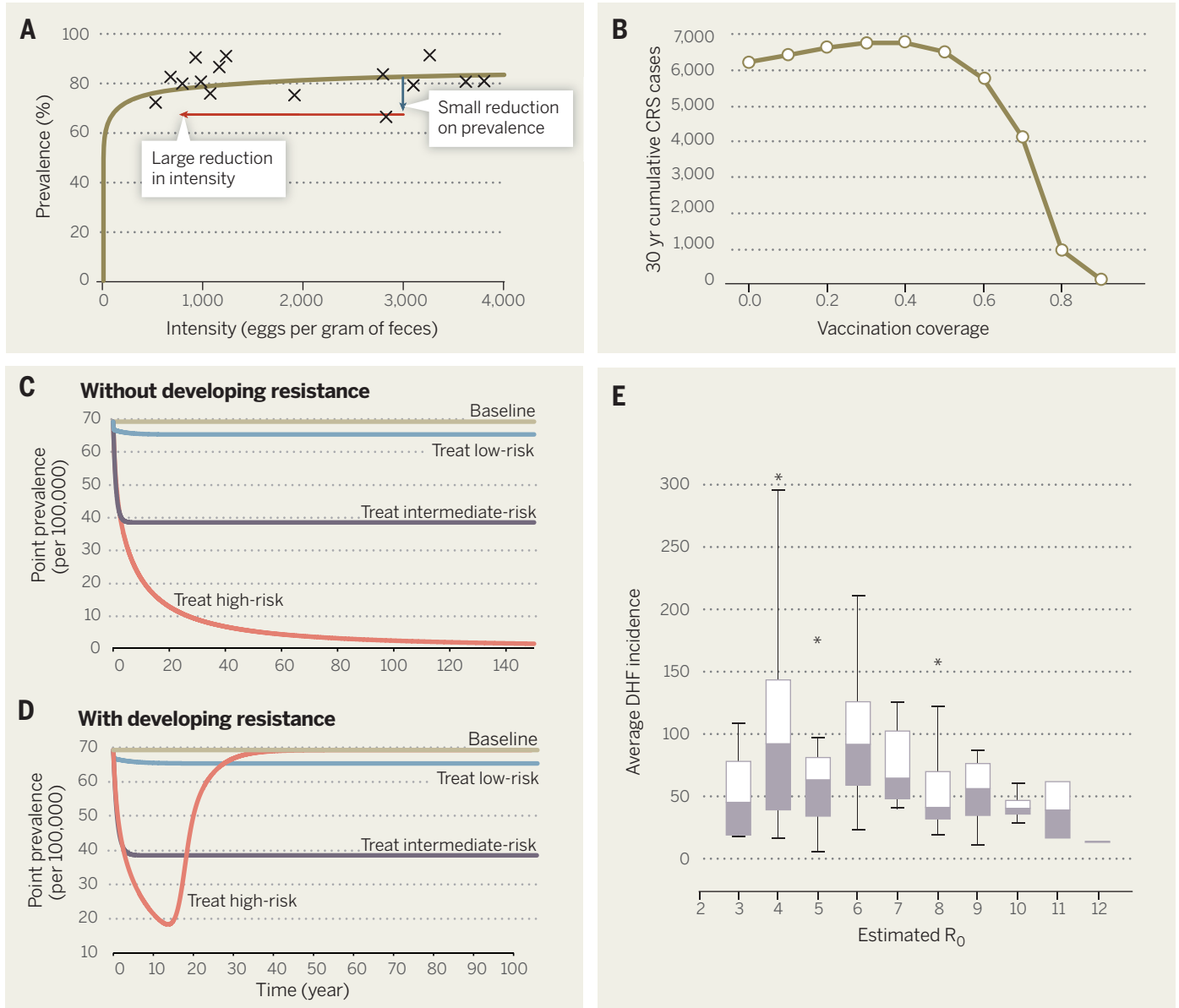
Fig. 2. Examples of counterintuitive effects of nonlinear infection dynamics.
